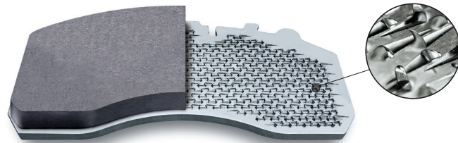
NRS™ Air Disc CV Pad
